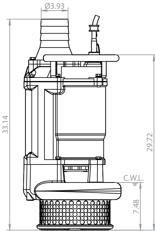
Dimensions in inches. C.W.L.: continuous running water level.
