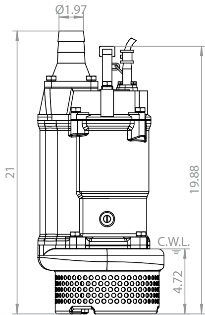
Dimensions in inches. C.W.L.: continuous running water level.
